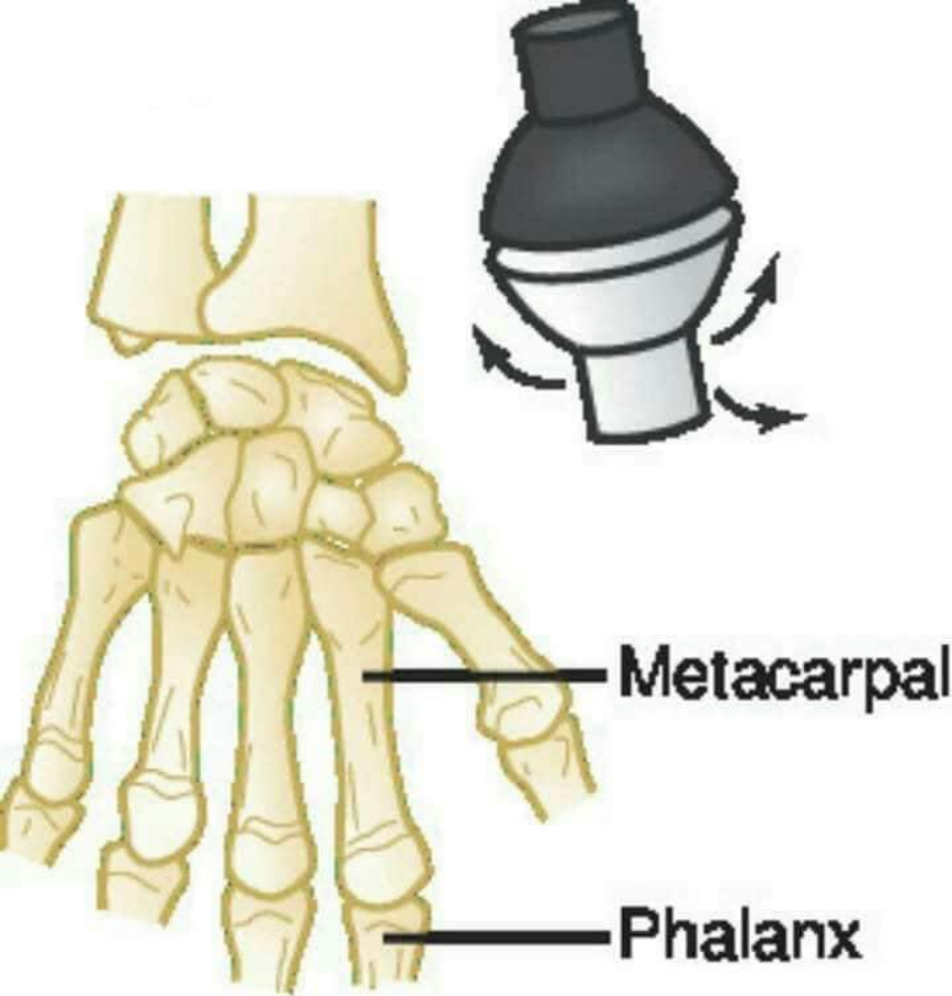
Condyloid joint
