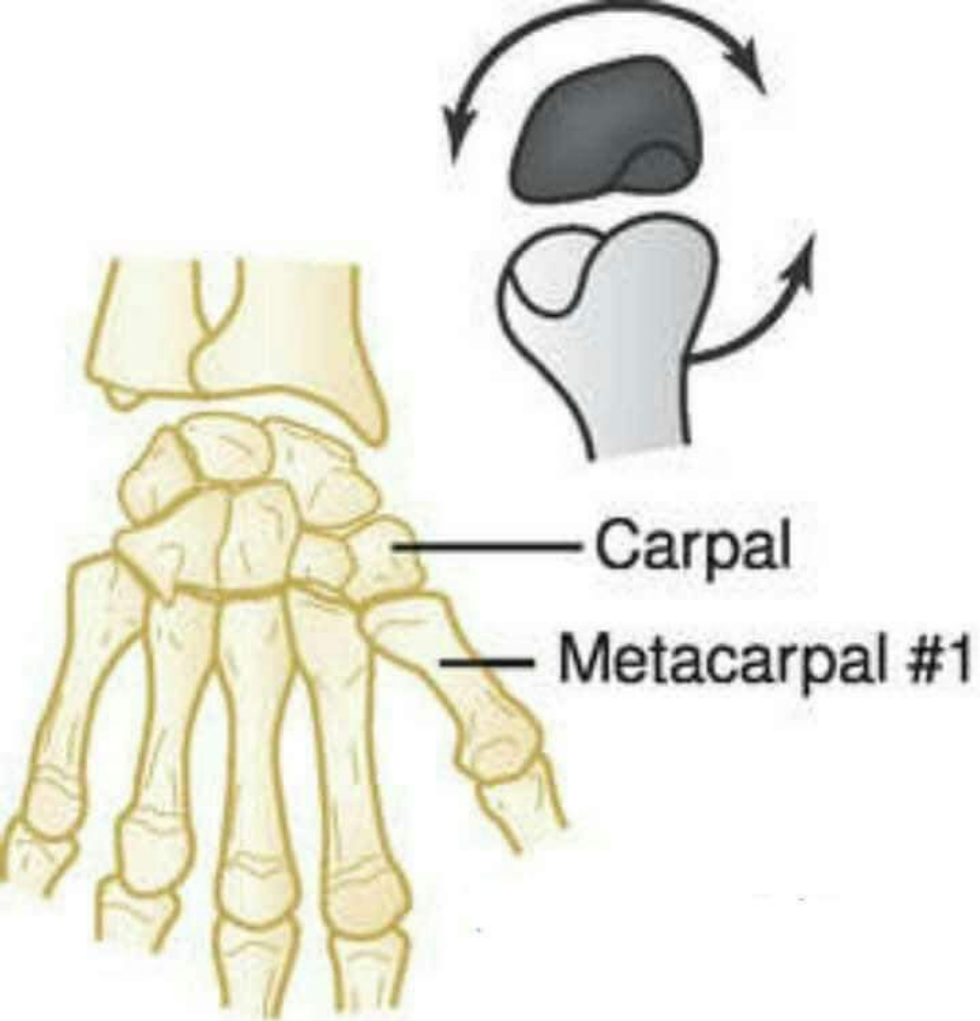
Saddle joint
