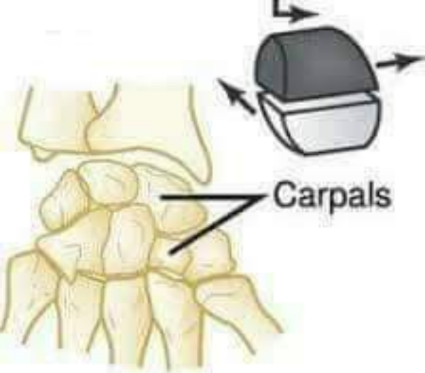
Plane joint
